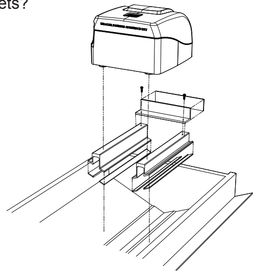
SKI ISO EXPLODED VIEW 2-C
